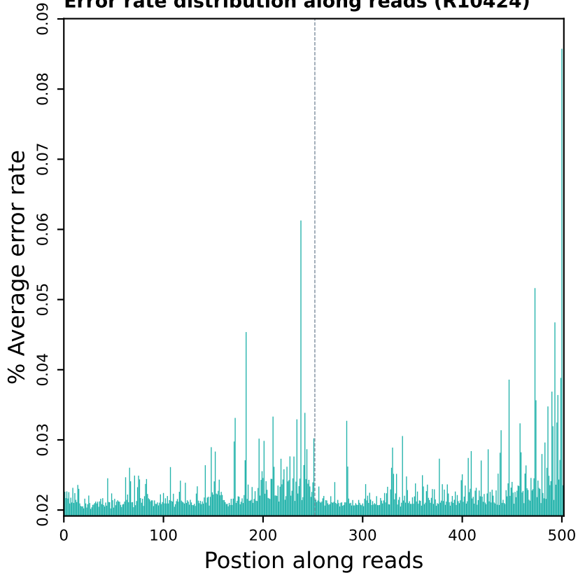
Error rate distribution along reads (R10424)
